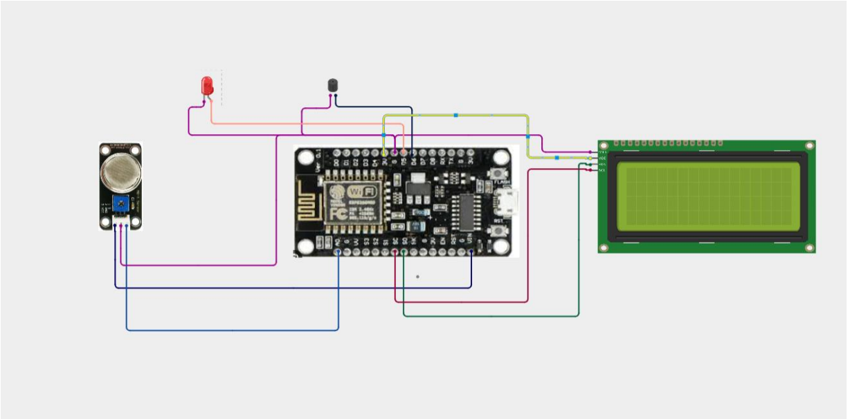
Fig. 2 Circuit wiring diagram
